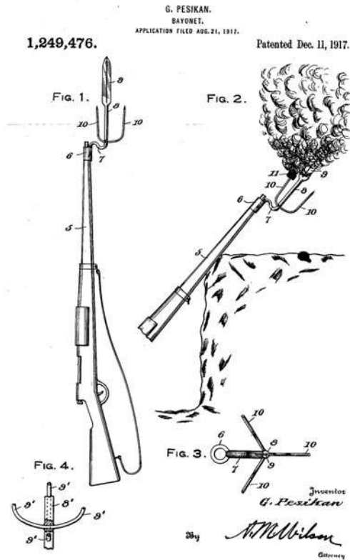
Bajuneta - Patent br. US1249476A
